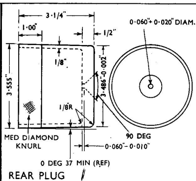
Fig. 29 Bore Plugs
