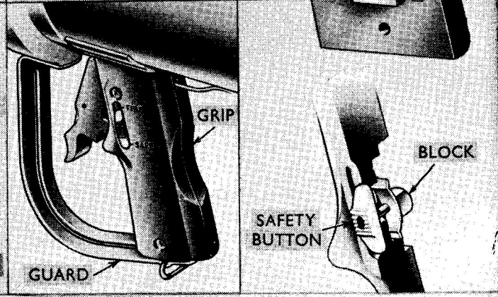
Fig. 8 Firing Mechanism
