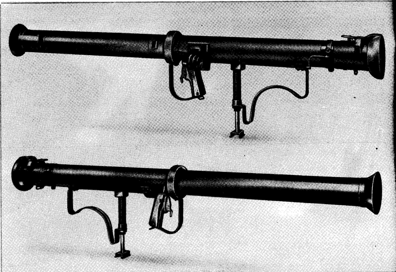
Frontispiece — 3.5 inch Rocket Launcher U.K. M20, MK. 2
