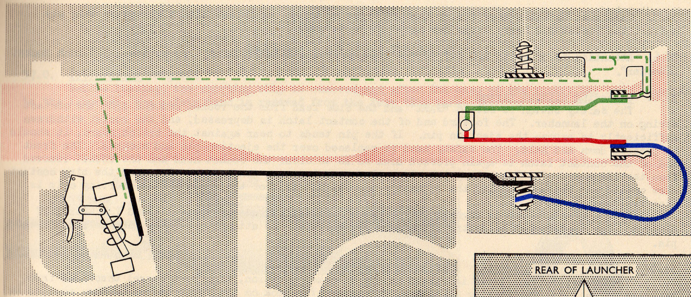
Fig. 20 Firing Circuit
