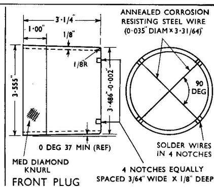
Fig. 29 Bore Plugs
