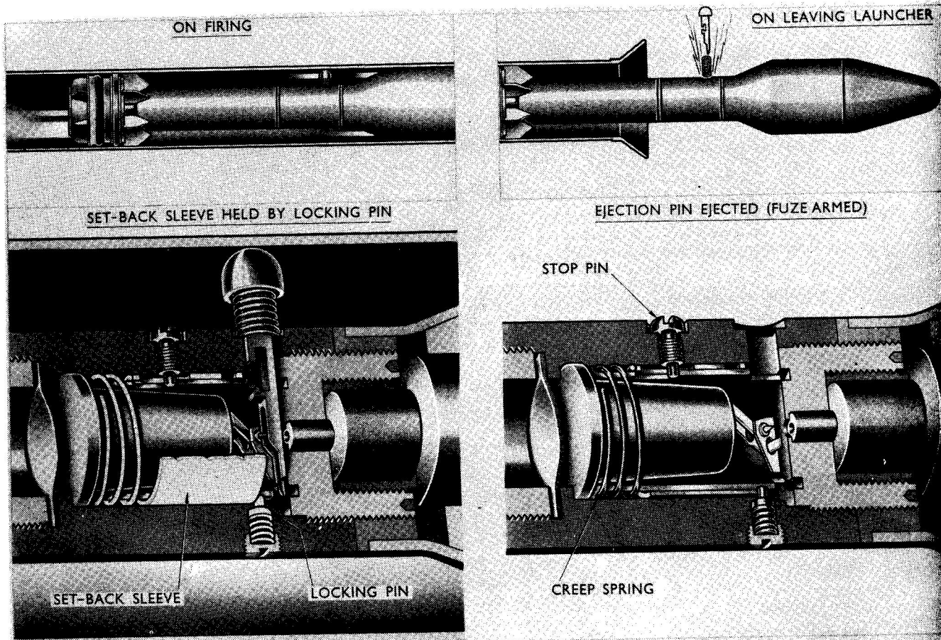
Fig. 25 Action of Fuze on Firing and During Flight
