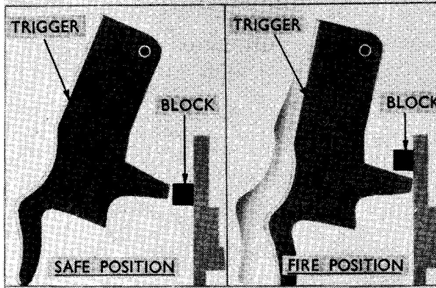
Fig. 8 Firing Mechanism
