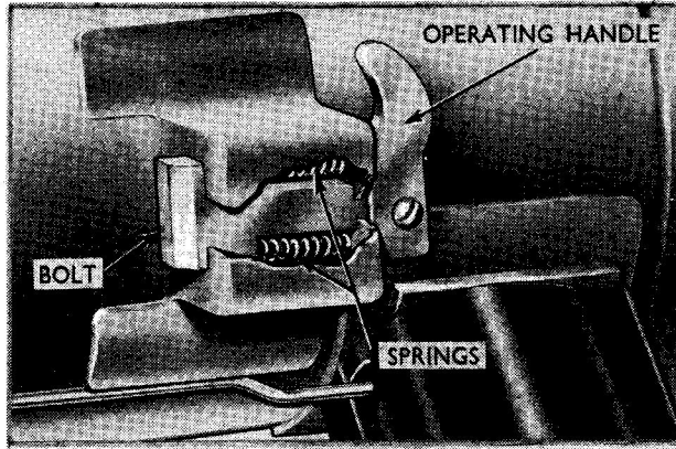
Fig. 7 Latch Bolt Assembly
