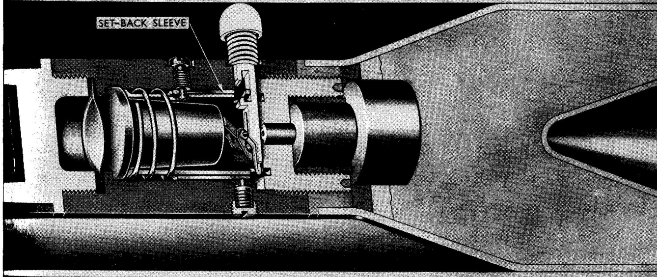
Fig. 24 Rocket completely Loaded
