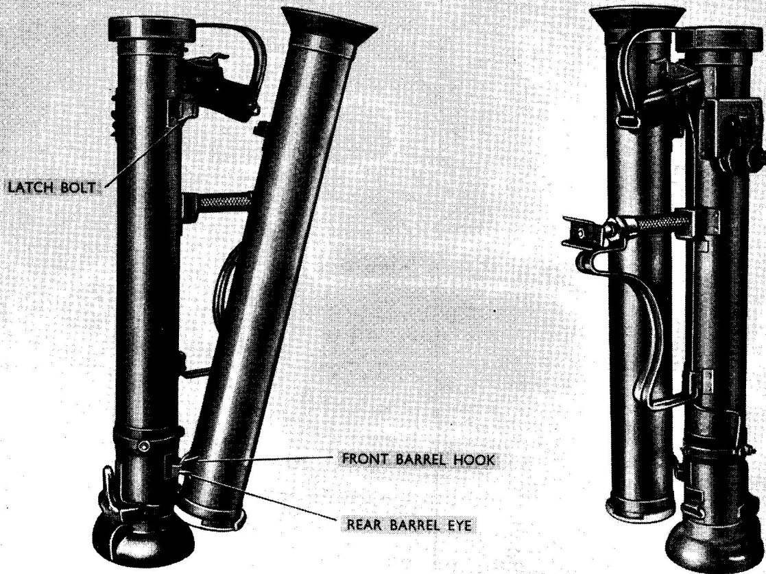
Fig. 2 The Barrel-Carrying Position
