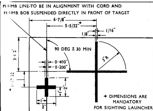
Fig. 28 Sight Testing Board
