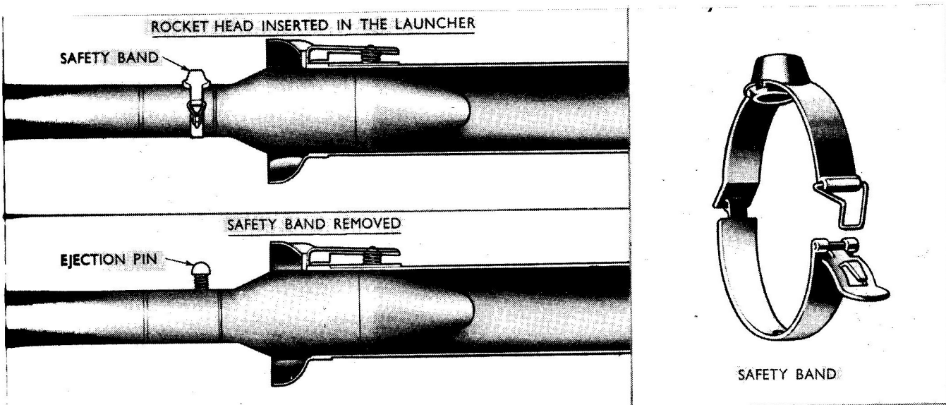
Fig. 22 Preparation for Loading
